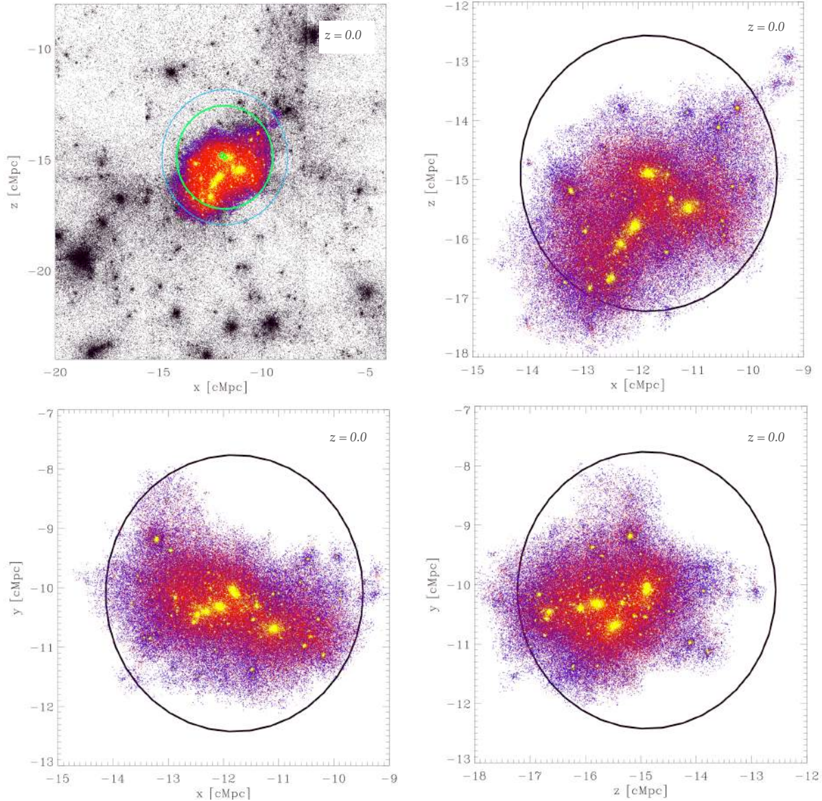
Figure 3.5: Projections of the internal structure of the main cluster in the region g1483463. In the upper left panel the green and blue circles represent R_{vir} and R_{200} as calculated by SUBFIND. In the rest of the figures the black circle stands for R_{vir} . The internal structure of this cluster does not show a dominating central galaxy but a chain of similar mass galaxies in the ranges 10^{11} - 10^{14} M_{\odot} . These are in turn surrounded by smaller satellite galaxies lying all over the cluster halo.
