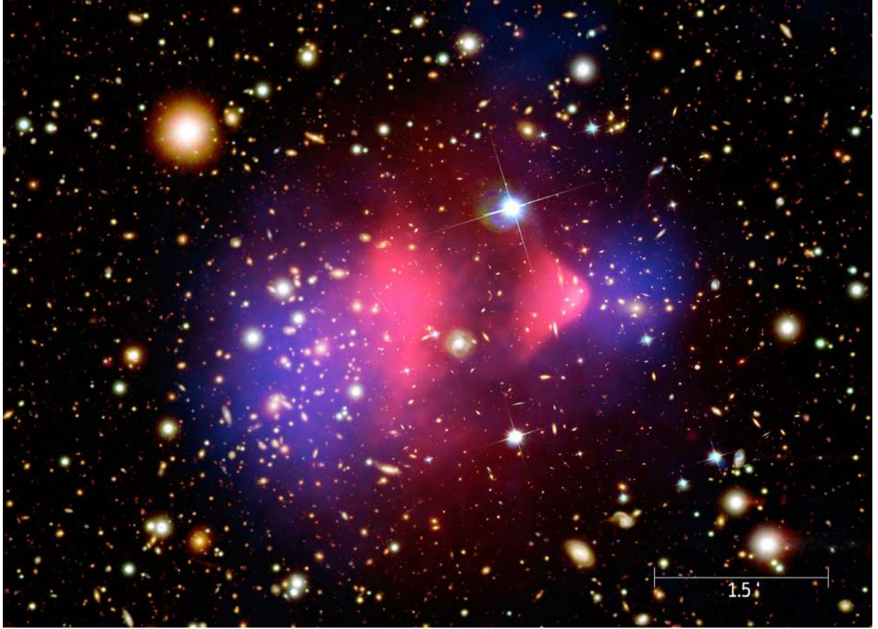
Figure 1.4: Composite image of the galaxy cluster 1E 0657-56, fondly known as the "bullet cluster". The optical image from the Magellan and the Hubble Space Telescope shows galaxies in orange and white in the background (credit: NASA/STScI; Magellan/U.Arizona/D.Clowe et al.) . Hot gas, which contains the bulk of the normal matter in the cluster, is shown by the Chandra X-ray image, which shows the hot intracluster gas (pink; credit: NASA/CXC/CfA/ M.Markevitch et al.). Gravitational lensing reveals the dark matter (blue; credit: NASA/STScI; ESO WFI; Magellan/U.Arizona/ D.Clowe et al.), which represents the dominant mass component of the structure.
