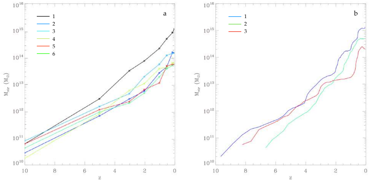
Figure 3.14: Evolution of virial masses through redshifts for the clusters in the Lagrangian regions g0272097 (left panel) and g1212639 (right panel). In both figures we observe several surpassings between halos. Some protoclusters with a higher mass rank at high redshifts end up as clusters with a lower mass rank at lower redshifts. Examples are halos 3 and 5 in the left panel and halos 1 and 2 in the right panel.
