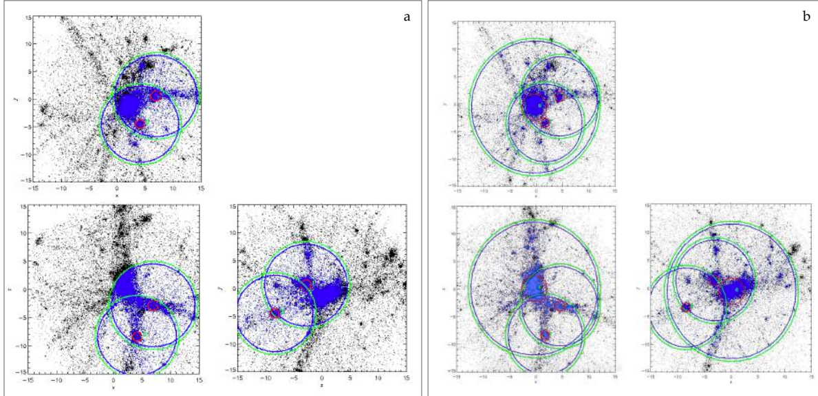
Figure 3.13: Both panels show the same Lagrangian region at same redshift. In the figure at the right SUBFIND was runned in serial mode and detected the three main overdensities. In the left panel we runned SUBFIND in parallel mode and it ignored the existence of the most massive halo.
