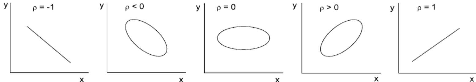
f(x,y) = \text{const} for different correlation coefficients (linear dependence: f(x,y) = f(y|x)f(x) with f(y|x) = \delta(y - (a + bx)) )
