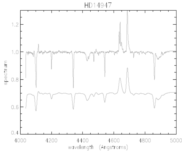
Figure 1.1: Top: optical spectrum of the hot supergiant HD14947, observed with high resolution. Bottom: same spectrum, observed with 8-times lower resolution (shifted by -0.3 ): the signal has been washed out.
