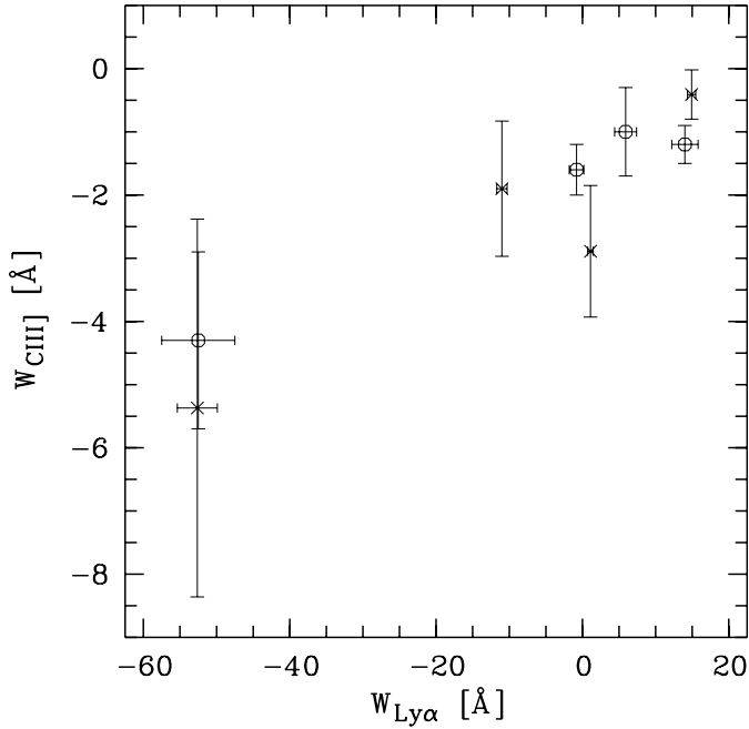
Fig. 19. The dependence of the strength of C III] \lambda\lambda 1907, 1909 on the Ly \alpha equivalent width. The open circles represent the values measured in the FDF composite spectra for different Ly \alpha strengths. For comparison the corresponding data from S03 are also included (crosses).
